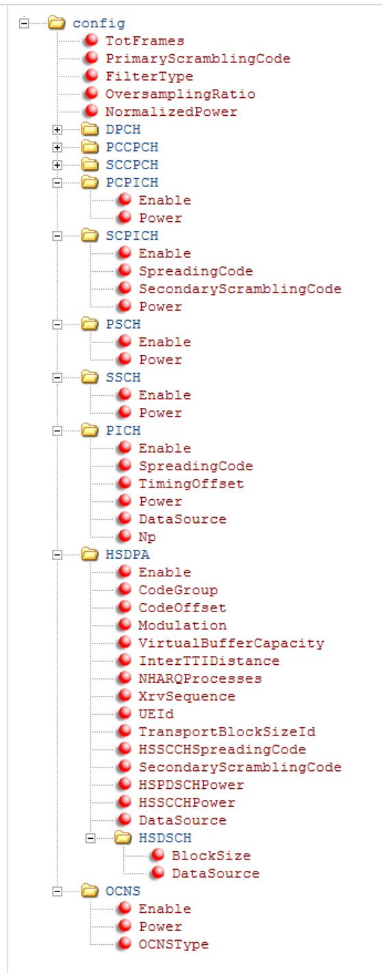
The config structure with PCPICH
